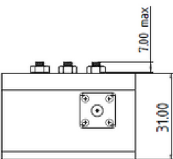
RIGHT VIEW
