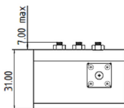
LEFT VIEW
